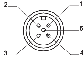
Round connector M 12 x 1 (5-pin)
